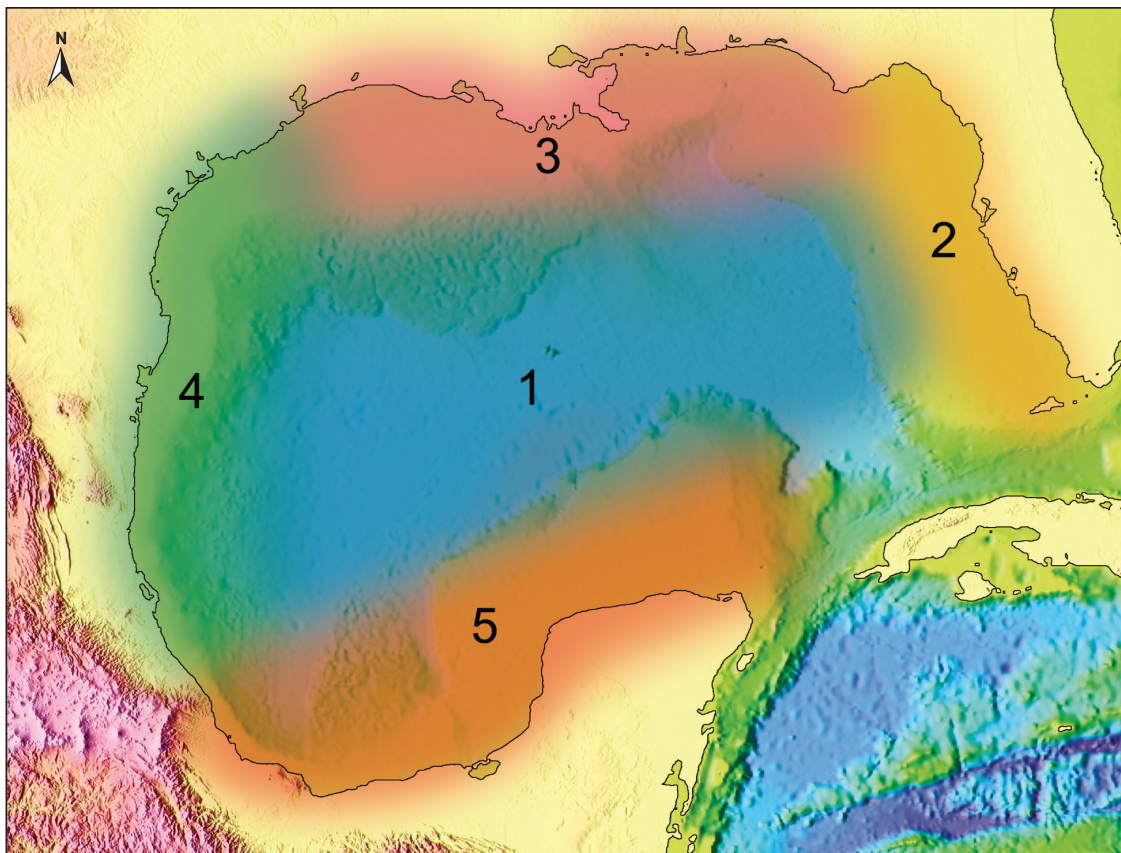
Figure 4. The Gulf of Mexico offers a variety of environments well suited for studying various aspects of carbon transport and related processes: (1) the open Gulf, (2) the West Florida shallow carbonate shelf, (3) the river-dominated northern shelf, (4) the narrow western shelf with its strong eddy-shelf interactions, and (5) the tropical Campeche Bay/Bank. Each region includes the watersheds of the streams and rivers that flow into the region's estuaries and onto the shelf.
