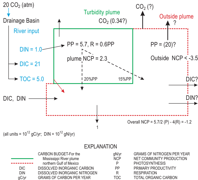
Figure 5. Carbon budget for the Mississippi River plume (green box) and northern Gulf of Mexico. Courtesy of Wei-Jun Cai.
